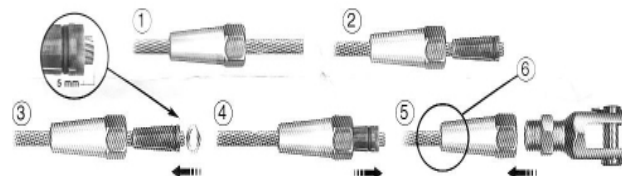
Jaw housing Caja Coopimorsetto
